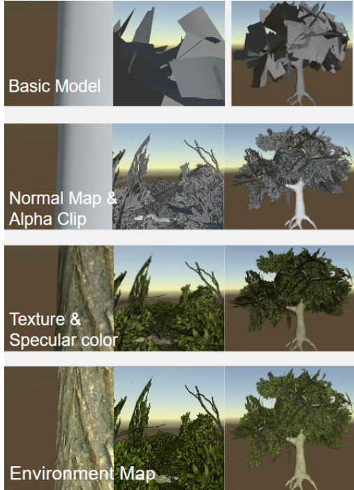
Figure 3. Rendering steps.
